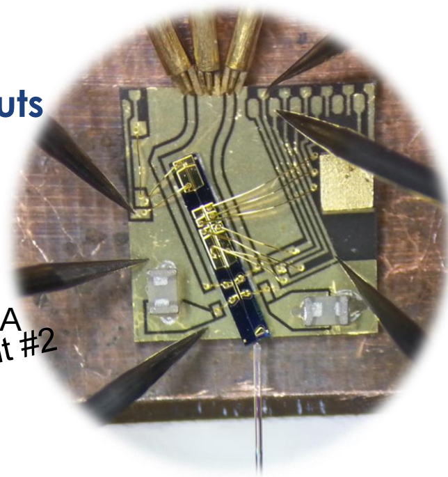
Fig. 1. Photograph of the device under test.
