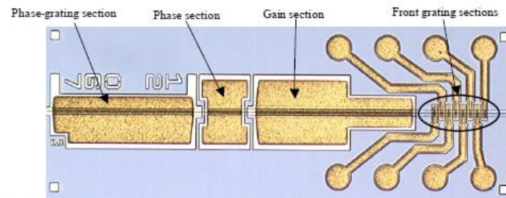
Figure 3.2: Top view of a DS-DBR laser chip.
