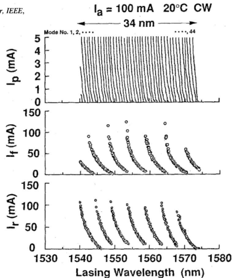
Fig. 12. Quasicontinuous wavelength tuning characteristics with three-tuning-current control.
